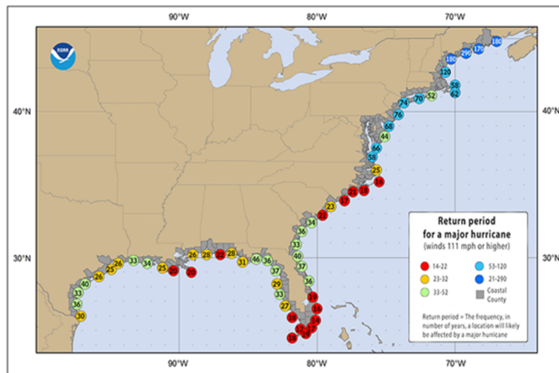
Figure A1. Return period (years) for major hurricanes for the coastal Eastern United States. Graphic provided by the National Oceanographic and Atmospheric Administration (NOAA).
