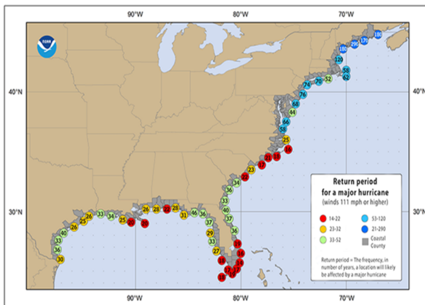
Figure A1. Return period (years) for major hurricanes for the coastal Eastern United States. Graphic provided by the National Oceanic and Atmospheric Administration (NOAA).
