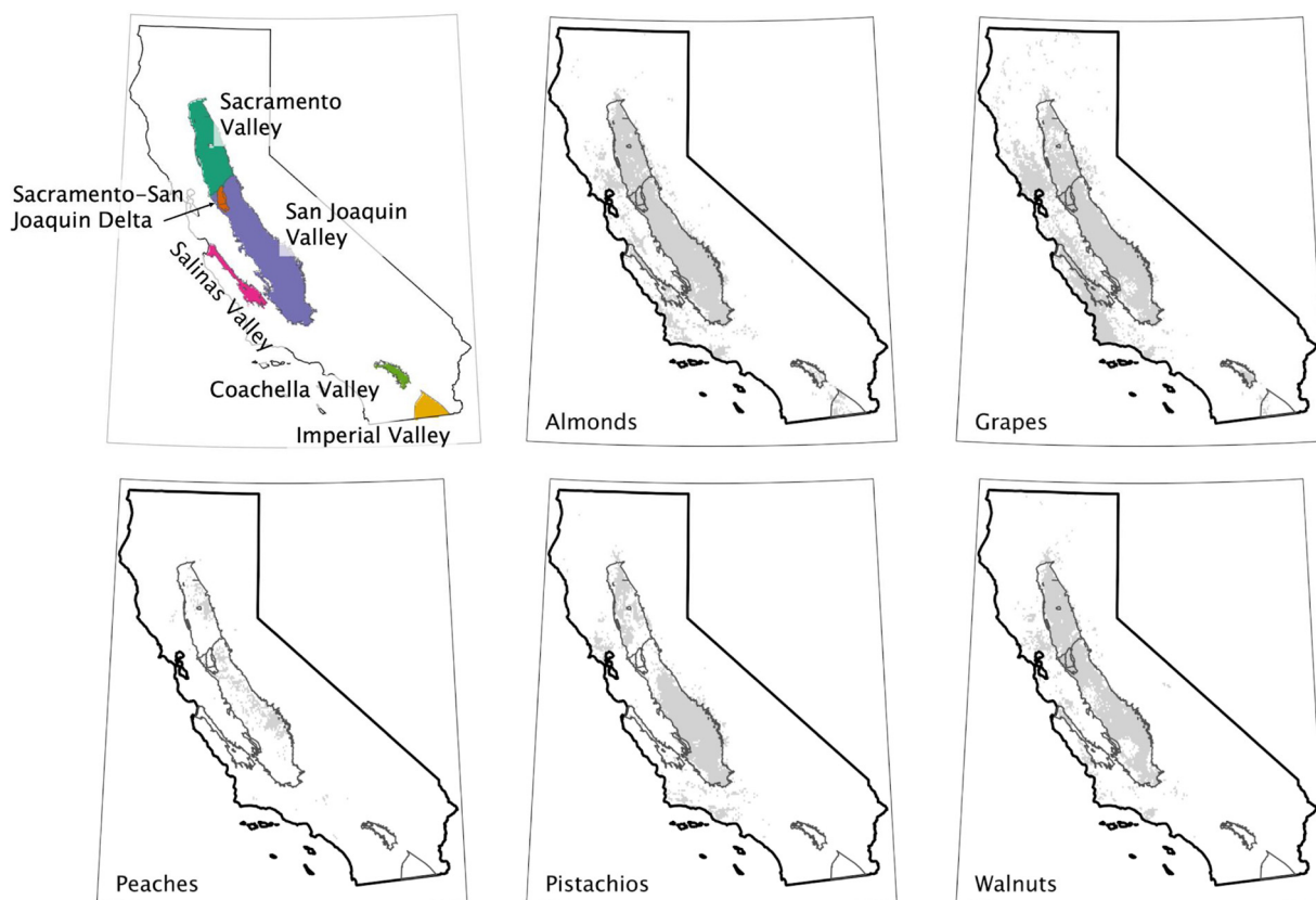
Fig. 1. Almonds, grapes, peaches, pistachios, and walnuts are largely concentrated within 6 California agricultural regions, with the majority of cultivation falling within the Sacramento and San Joaquin Valleys and Delta, which collectively comprise California's Central Valley. Grapes are a notable exception, with significant cultivation of winegrapes occurring in coastal hills south and west of the Salinas Valley, and west of the Sacramento Valley.
