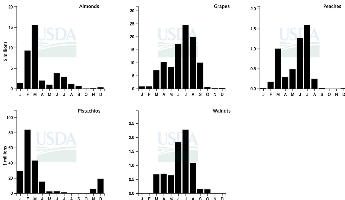
Fig. 3. Total crop losses (y-axis) by month (x-axis) over the 1989–2017 period, where the cause of loss was listed as “Heat.” Losses are represented by insurance indemnity payments in millions of dollars. Graphs downloaded from AgRisk Viewer [7].
