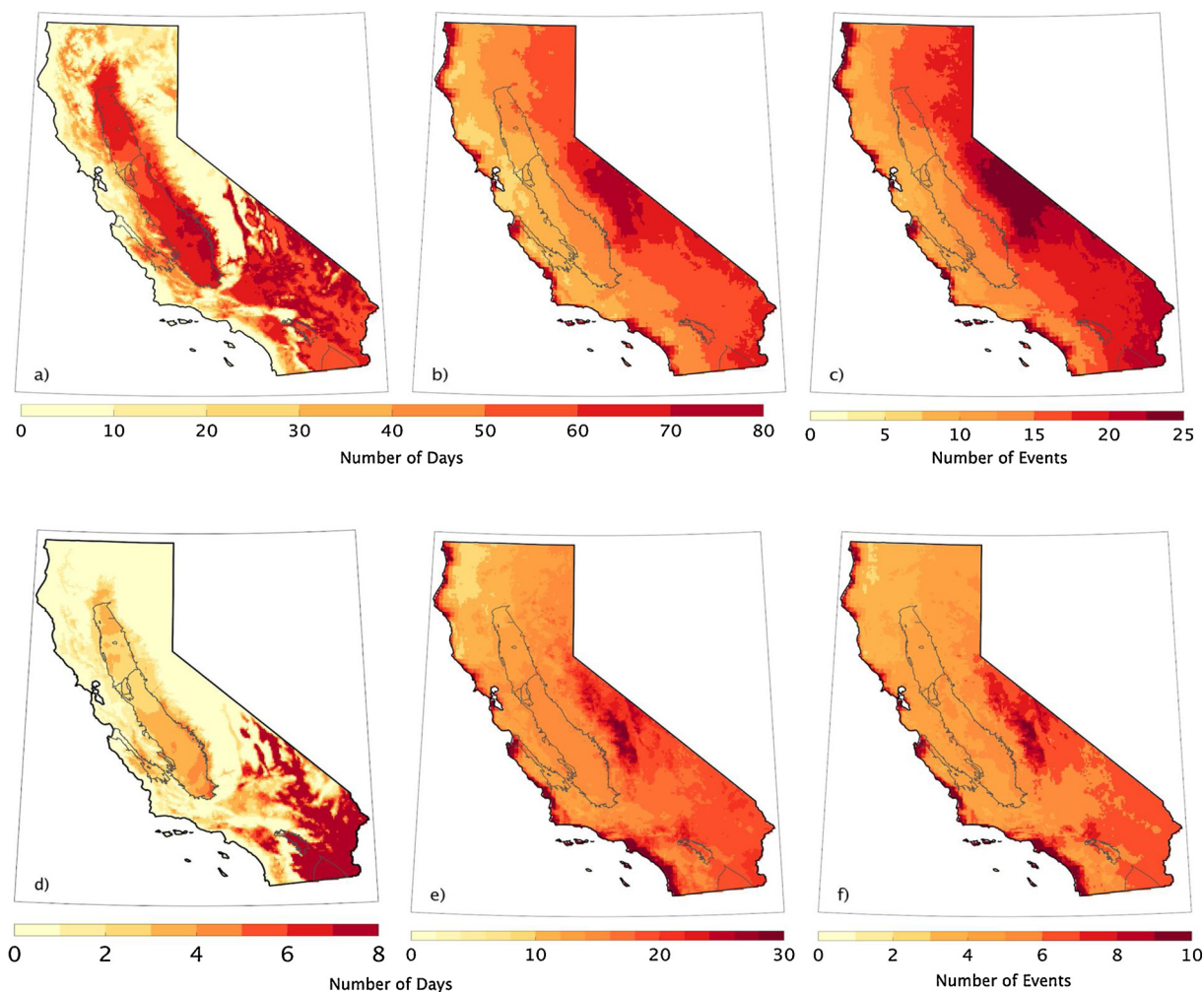
Fig. 2. The projected change between the observed contemporary (1981–2010) and modeled future (2070–2099, RCP 8.5) average annual number of (a) warm-season days with T_{max} > 38^{\circ}C , (b) warm-season days with T_{max} > 98 th percentile of observed 1981–2010 annual daily T_{max} , (c) warm-season 3-day heatwave events with T_{max} > 98 th percentile of observed 1981–2010 annual daily T_{max} (d) cool-season days with T_{max} > 38^{\circ}C , (e) cool-season days with T_{max} > 98 th percentile of observed 1981–2010 annual daily T_{max} , and (f) cool-season 3-day heatwave events with T_{max} > 98 th percentile of observed 1981–2010 annual daily T_{max} , Where the warm (cool) season is defined as April–September (October–March).
