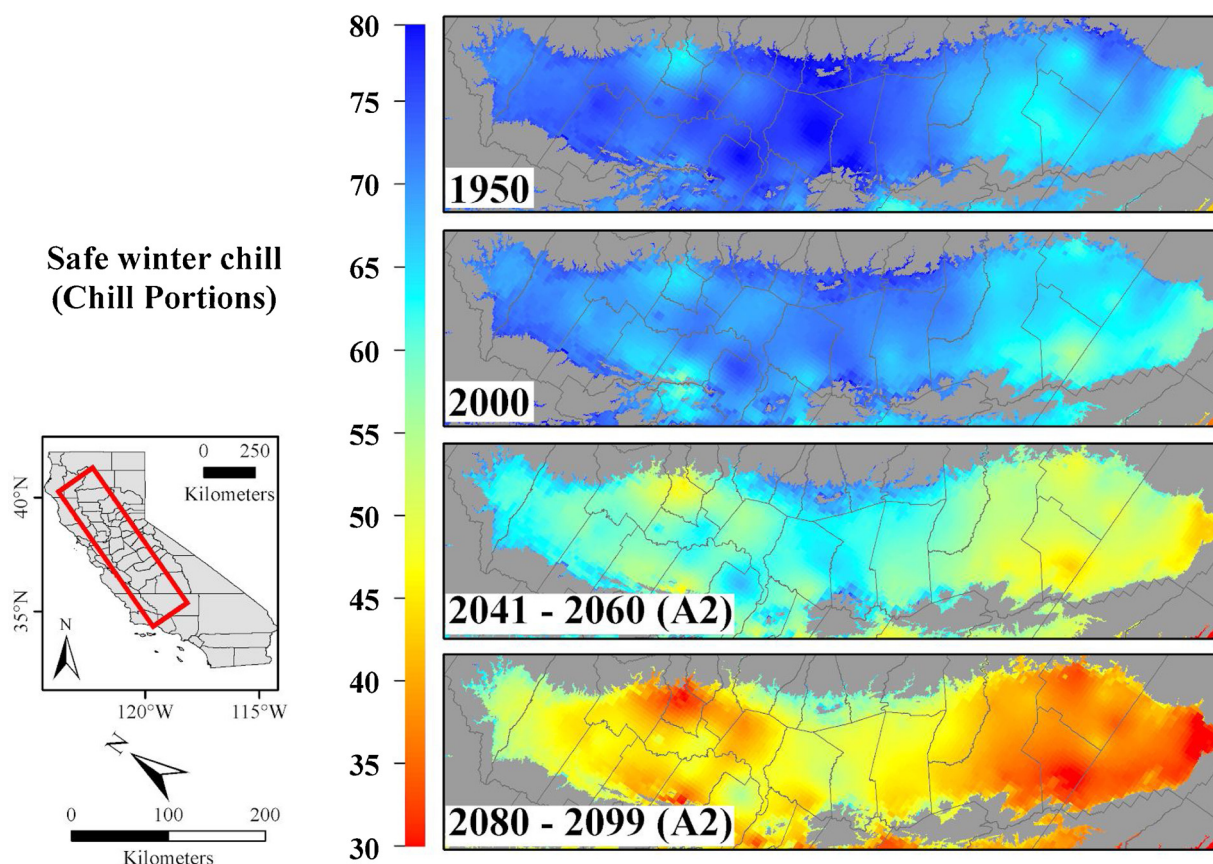
Fig. 4. Changes in the 10th quantile of winter chill accumulation over the Central Valley of California under modeled historic and future climate scenarios [56].
